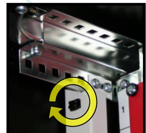
Secure baffle in position by rotating fixing through 90°
