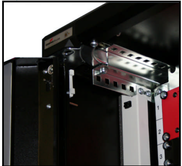
Access Cabinet 600mm wide Vertical Brush Strip Baffle Finished – Light Grey NCS 1502-Y
